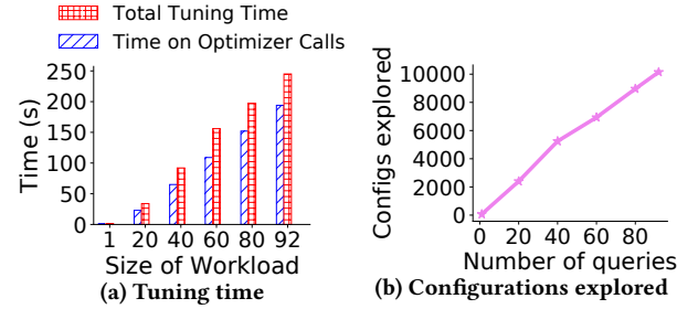
Figure 2: Scalability challenges in index tuning (TPC-DS workload)
