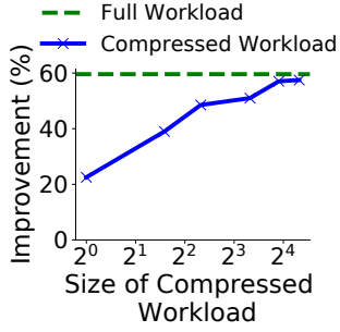
Figure 3: Impact of workload compression (TPC-DS workload)
