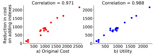
Figure 5: Relationship between utility and reduction in cost due to indexes when each query is tuned independently in the TPC-H workload. a) Utility is set to the original cost of the query, b) Utility considers both original cost and statistics such as selectivity of filter and join columns. Each point in the charts represents one query in the workload.
