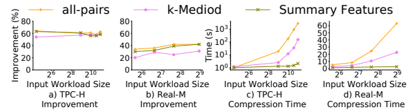
Figure 11: Comparing summary-features based algorithm with all-pairs and k -mediod [11] algorithms.
