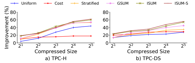
Figure 15: Comparing compression algorithms using DEXTER on PostgreSQL
