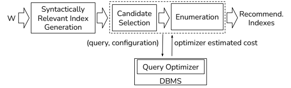
Figure 1: A typical architecture of index advisor as described in [14]
